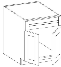
Vanity Sink Base Double Doors
